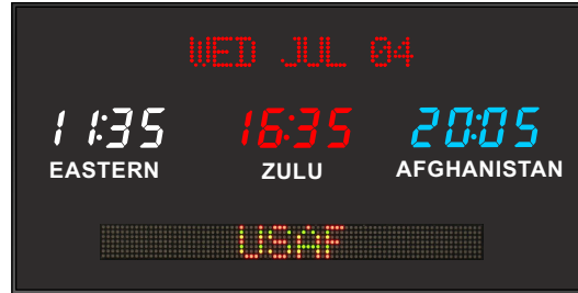
Model 689L - 2.5" time, 1.0" vinyl zone labels, 2.0" 10 character date 2.0" dot matrix message display 24" wide, 3 zones
