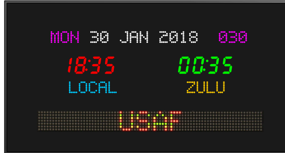
Model 6789P - 1.8" time, 1.2" zone labels, 1.2" 20 character date 2.0" dot matrix message display 24" wide, 2 zones
